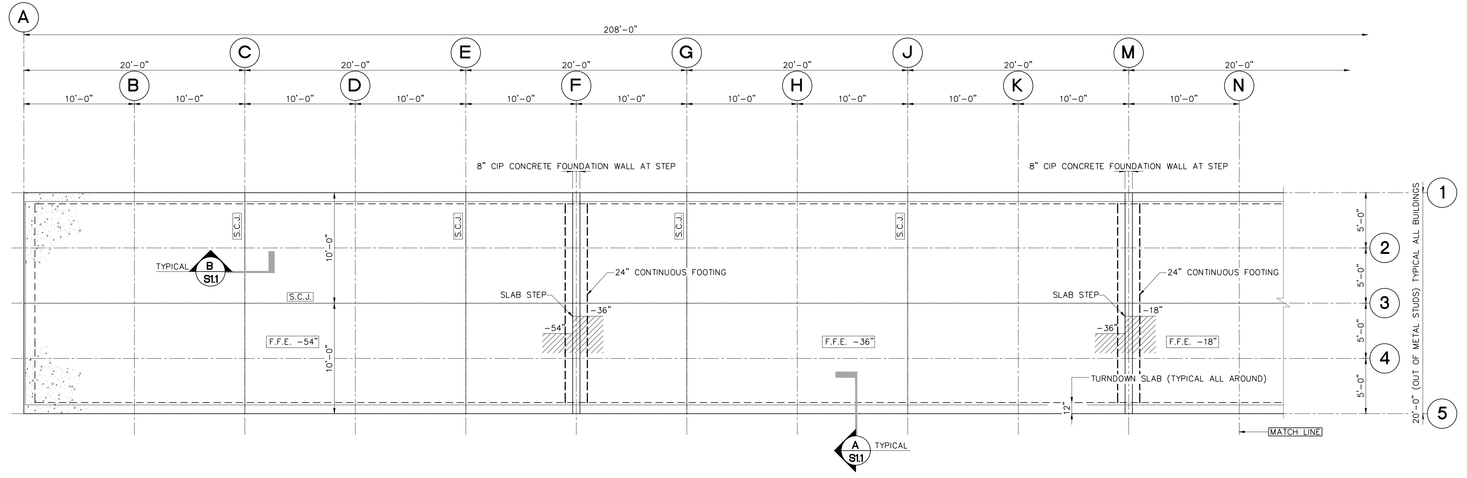
1 PLAN - BUILDING "B" FOUNDATION (208'x20') (PARTIAL) S1.1B 3/16"=1'-0" PROJECT NORTH
