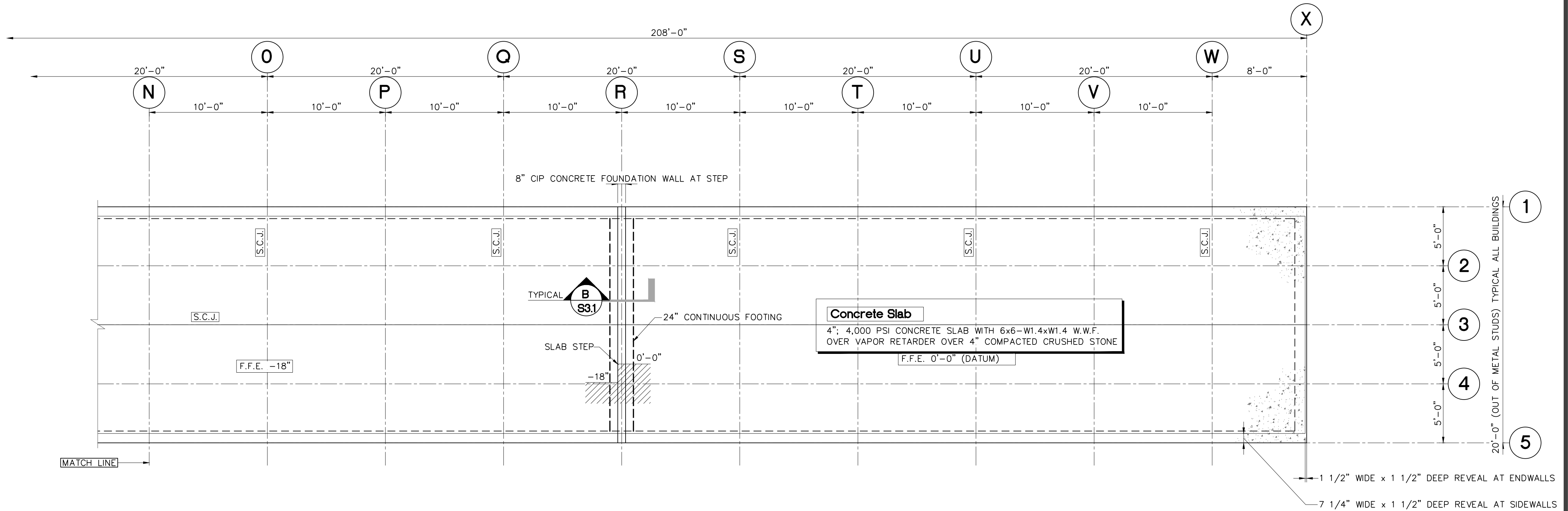
2 PLAN - BUILDING "B" FOUNDATION (208'x20') CONTINUED S1.1B 3/16"=1'-0" PROJECT NORTH
