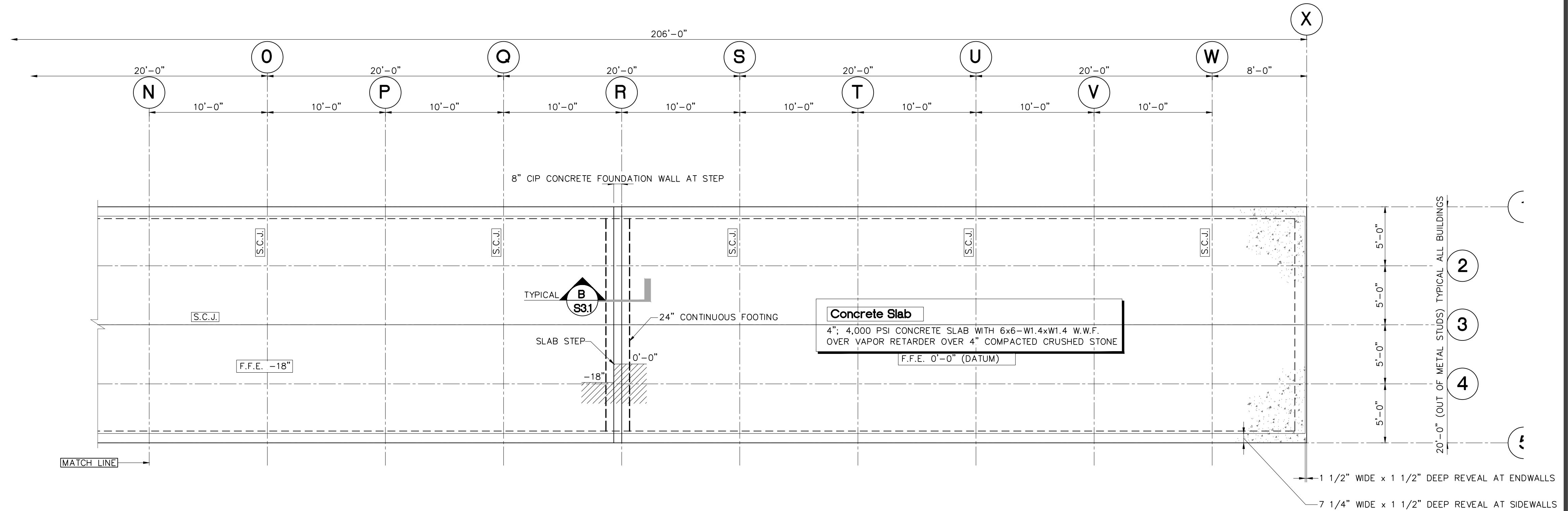
2 PLAN - BUILDING "C" FOUNDATION (206'x20') CONTINUED S1.1C 3/16"=1'-0" PROJECT NORTH
