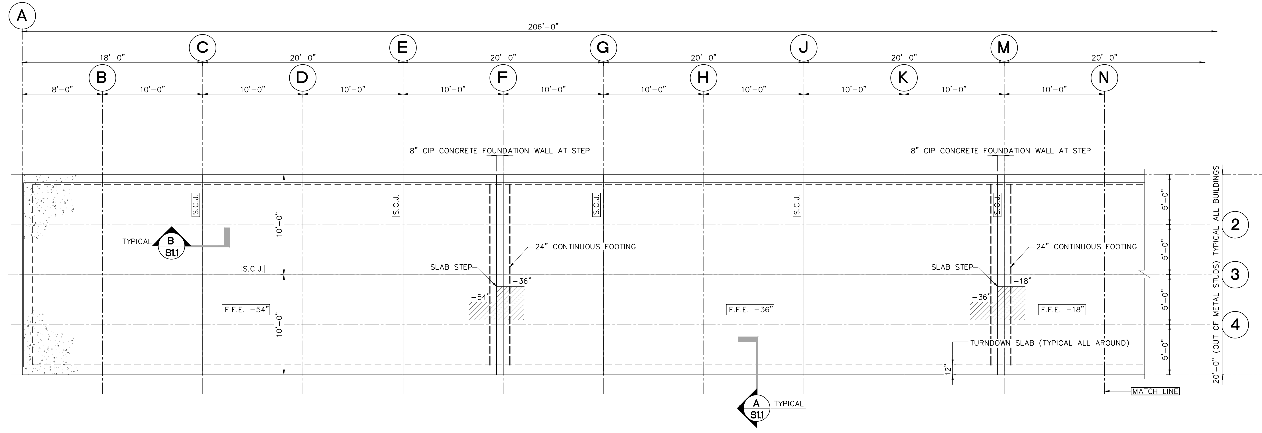
1 PLAN - BUILDING "C" FOUNDATION (206'x20') (PARTIAL) S1.1C 3/16"=1'-0" PROJECT NORTH
