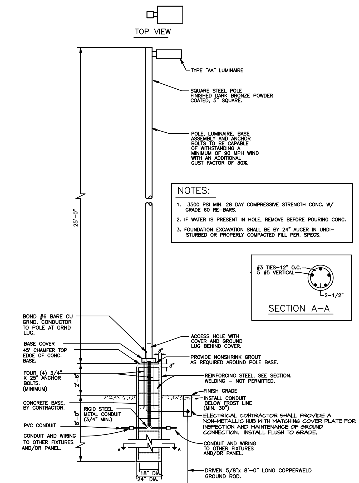
LIGHTING STANDARD DETAIL
