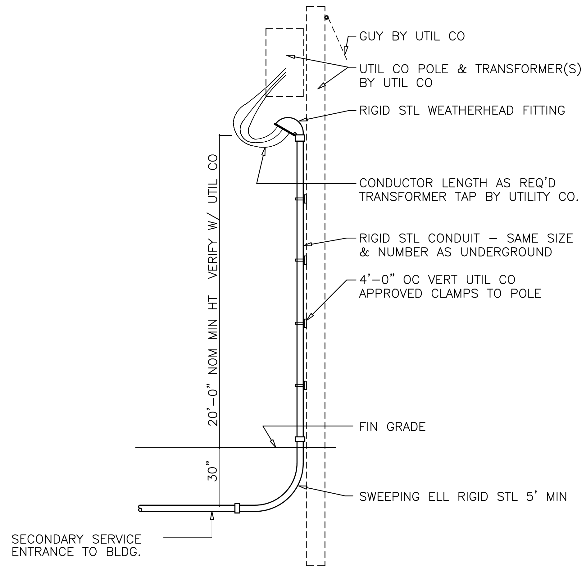
POLE MOUNTED TRANSFORMER DETAIL
