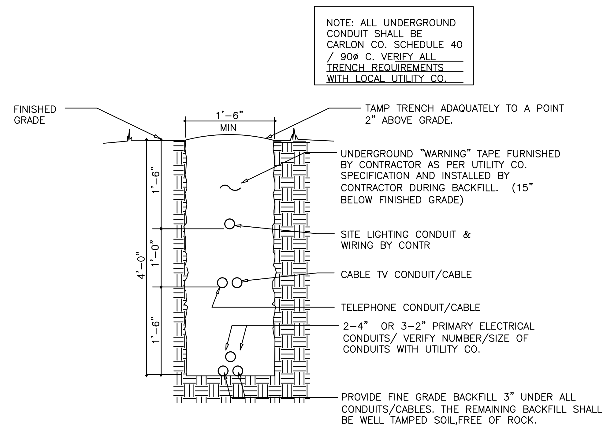
ELECTRICAL UTILITY TRENCH DETAIL
