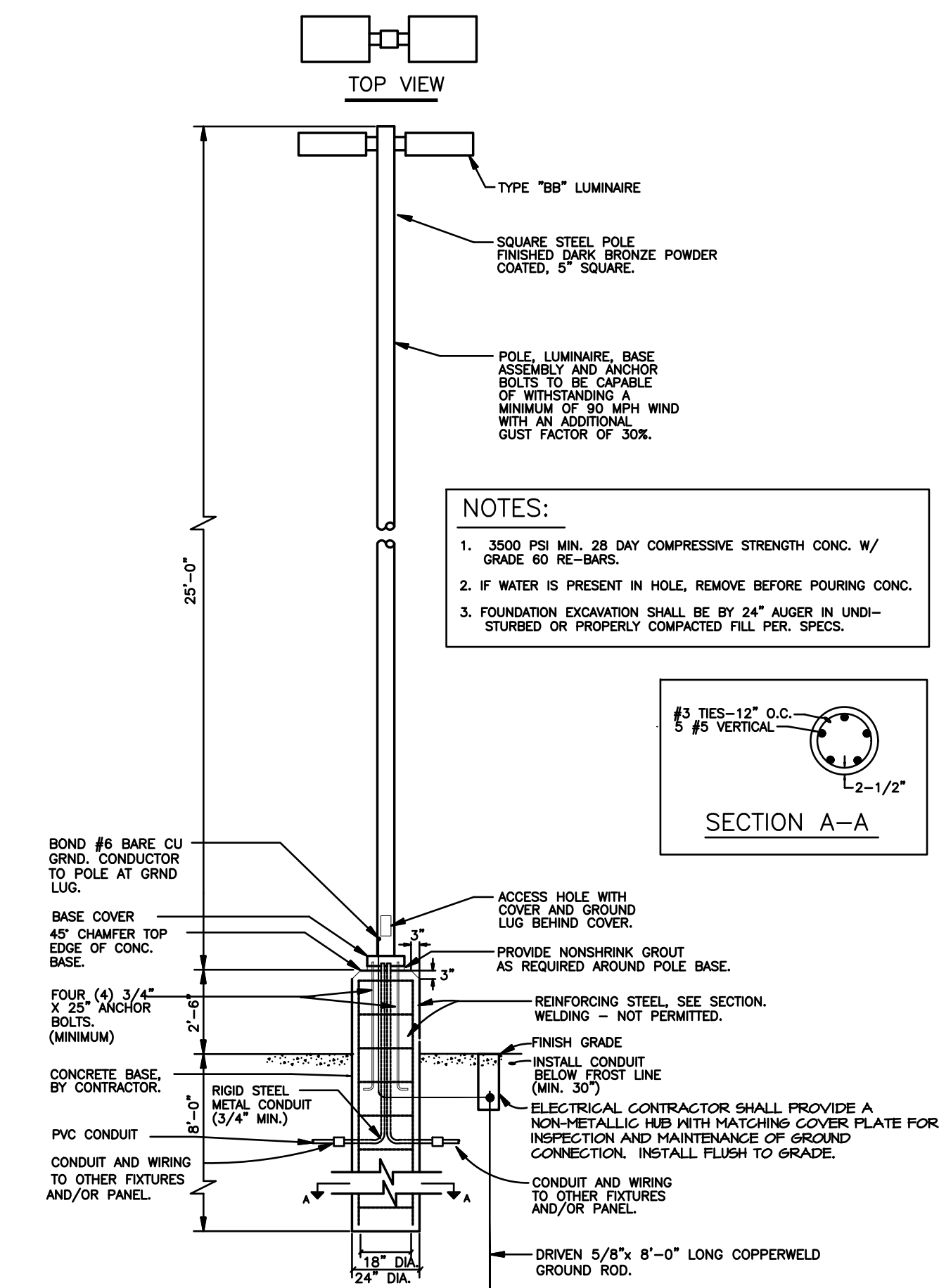
LIGHTING STANDARD DETAIL
