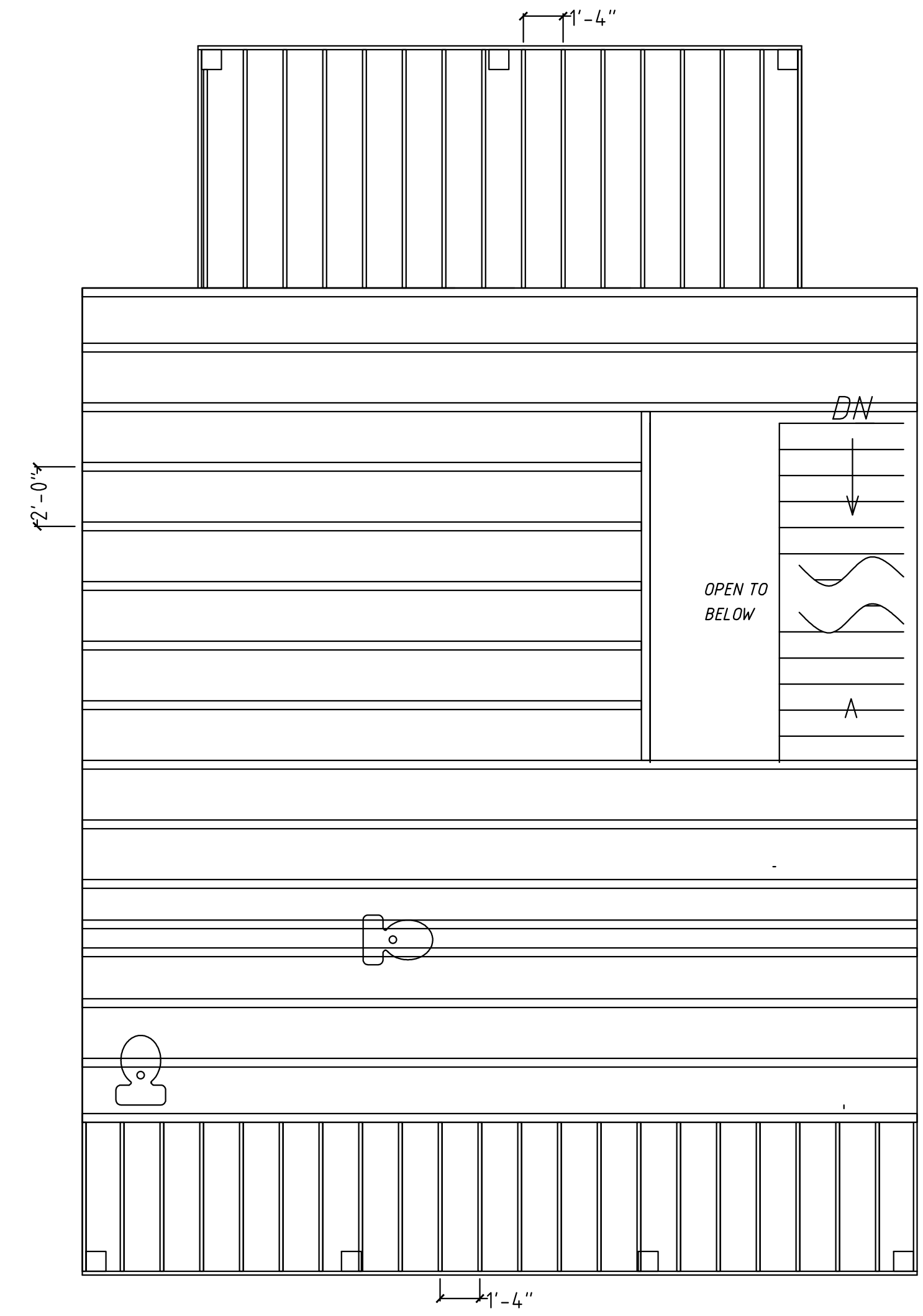
2nd FLOOR TRUSSES
