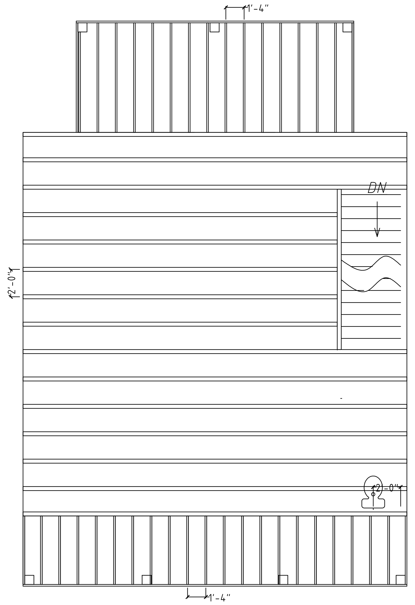
1st FLOOR TRUSSES
